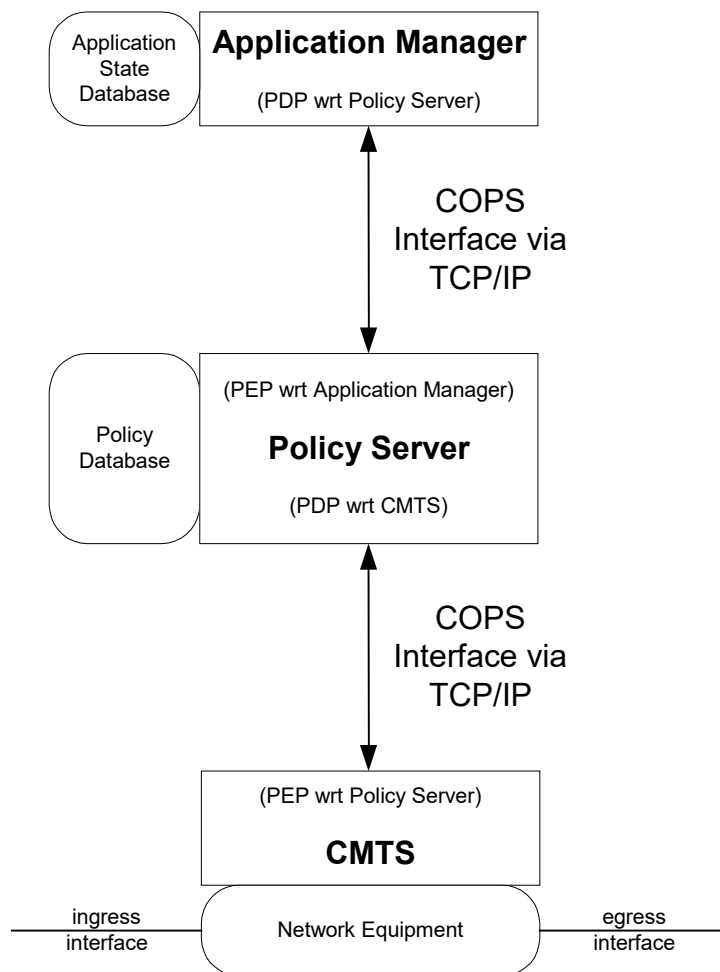
Figure 4 - QoS Admission Control Layout
