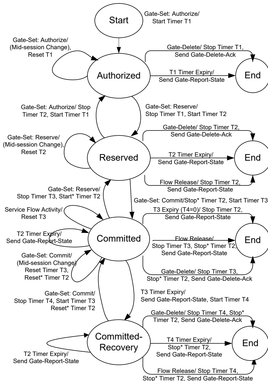
Figure 3 - Gate State Transitions
