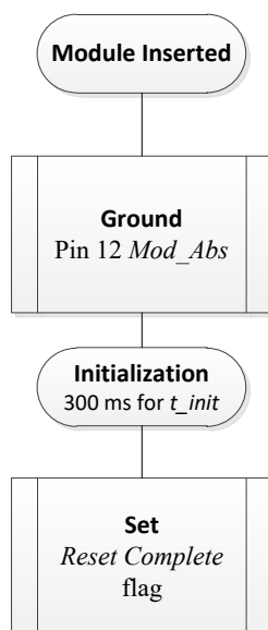
Figure 3 – PXFP-WDM Module Boot Sequence
