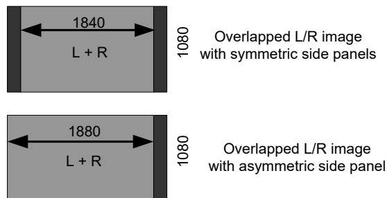
Figure 10 - HIT-adjusted image after cropping and side panels added
