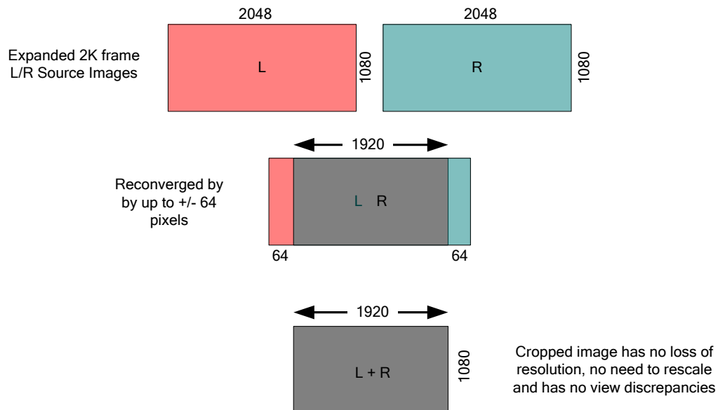
Figure 13 - Maximum HIT-adjustment of image using 2K format as source with 1920x1080 final output size after cropping
