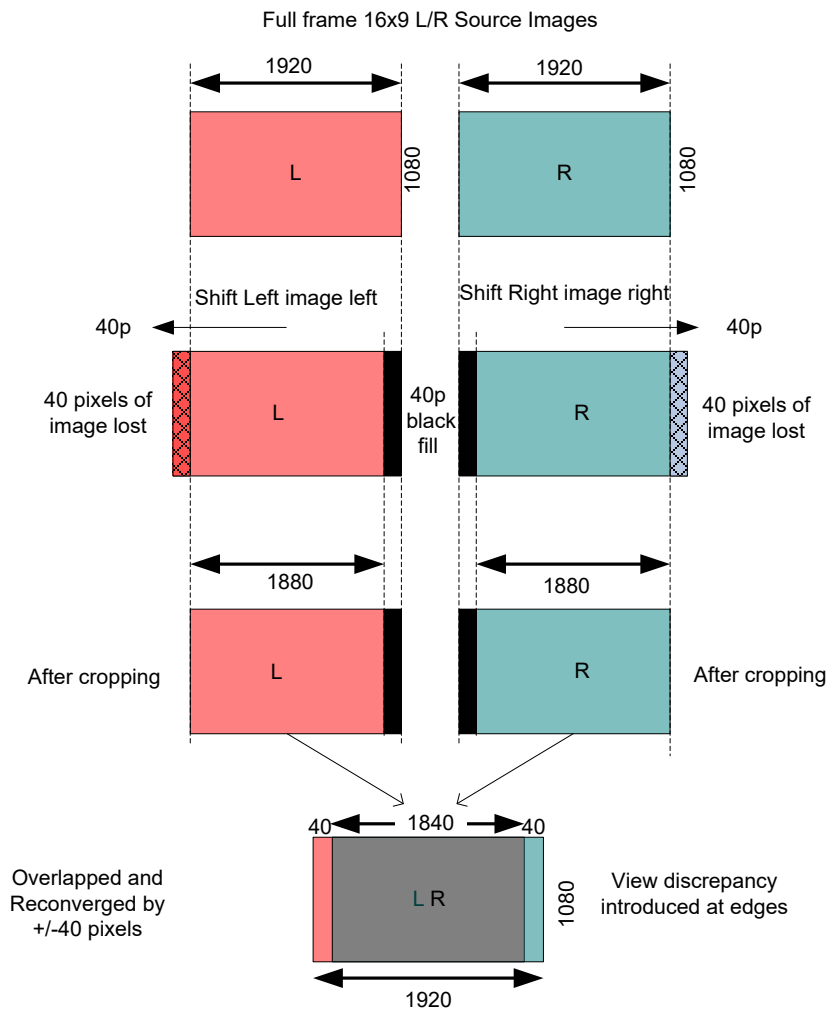
Figure 6 - Symmetric HIT adjustments with view discrepancies
