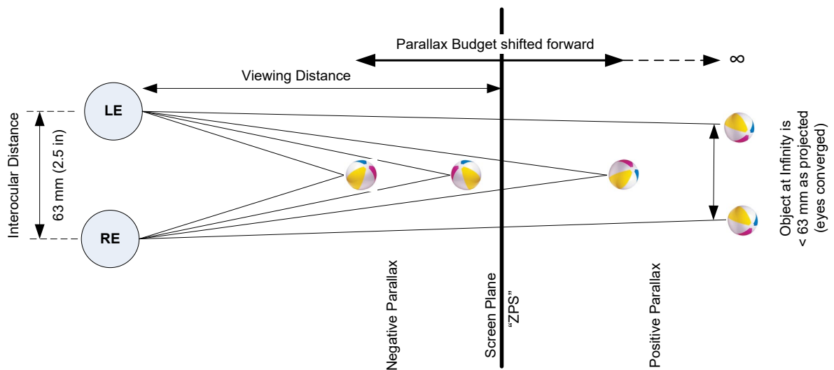
Figure 4 - Parallax budget shifted forward
