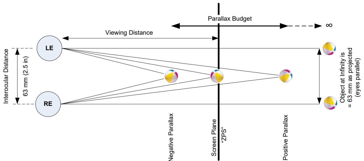
Figure 2 - The effects of the stereographer's parallax budget in relationship to the screen plane
