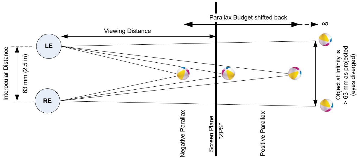
Figure 3 - Excessive positive parallax and divergence
