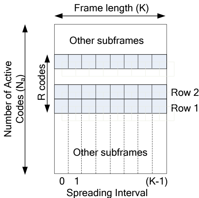
Figure 6–18 - Subframe structure
