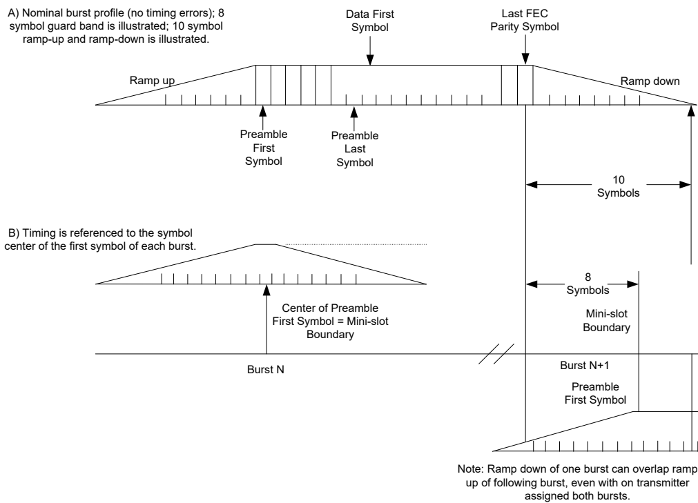
Figure 6–31 - Nominal TDMA Burst Timing
