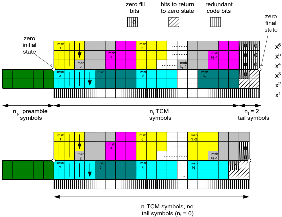
Figure 6-11 - Example Byte to Bit Assignment for 64-QAM
