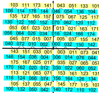
Figure 6-28 - 64-QAM and 128-QAM TCM Symbol Mapping
