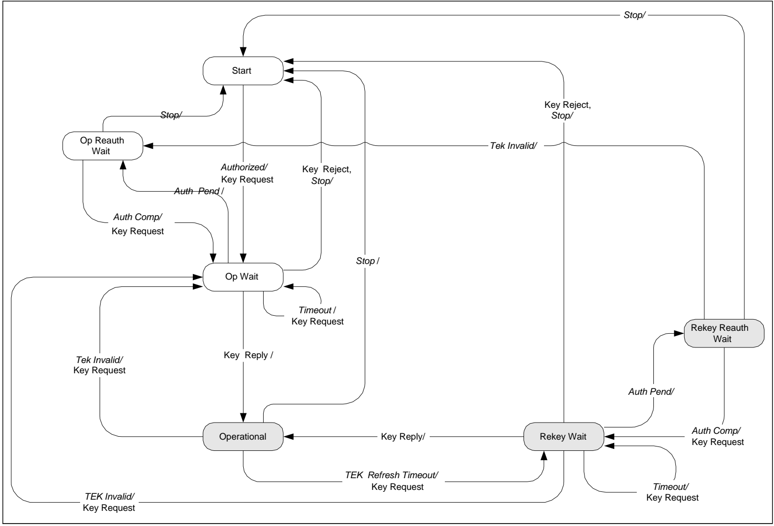
Figure 4-2. TEK State Machine Flow Diagram
