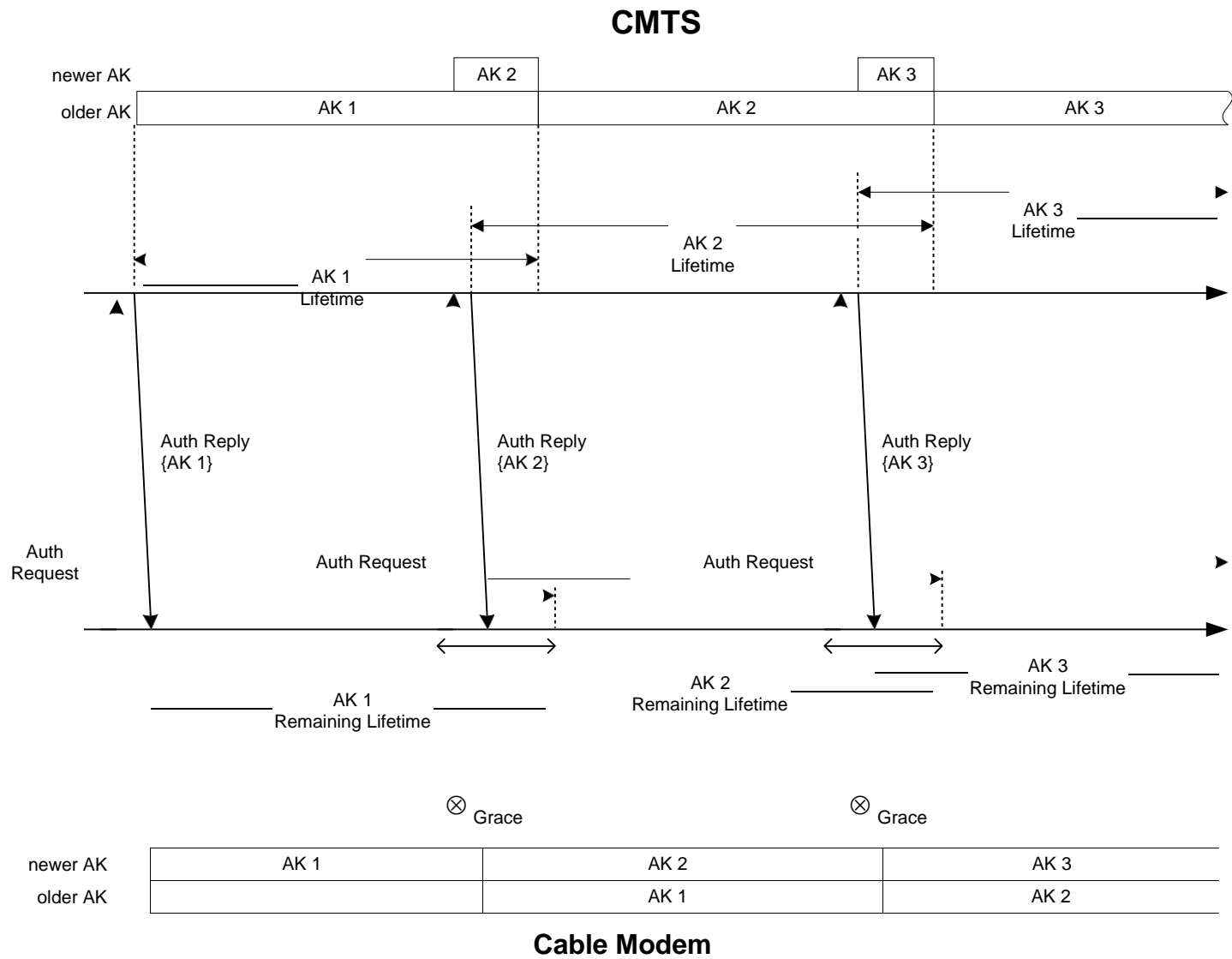
Figure 6-1. Authorization Key Management in CMTS and CM
