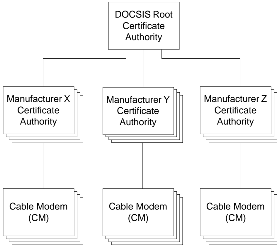
Figure 9-2. The Distributed Model of the DOCSIS Certificate Management Architecture
