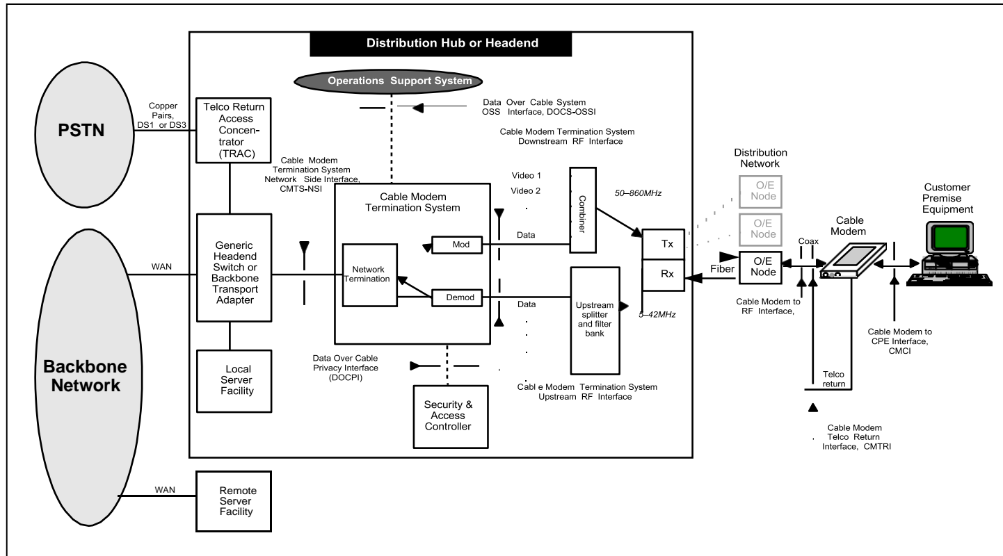
Figure 1-2. Data-over-Cable Reference Architecture
