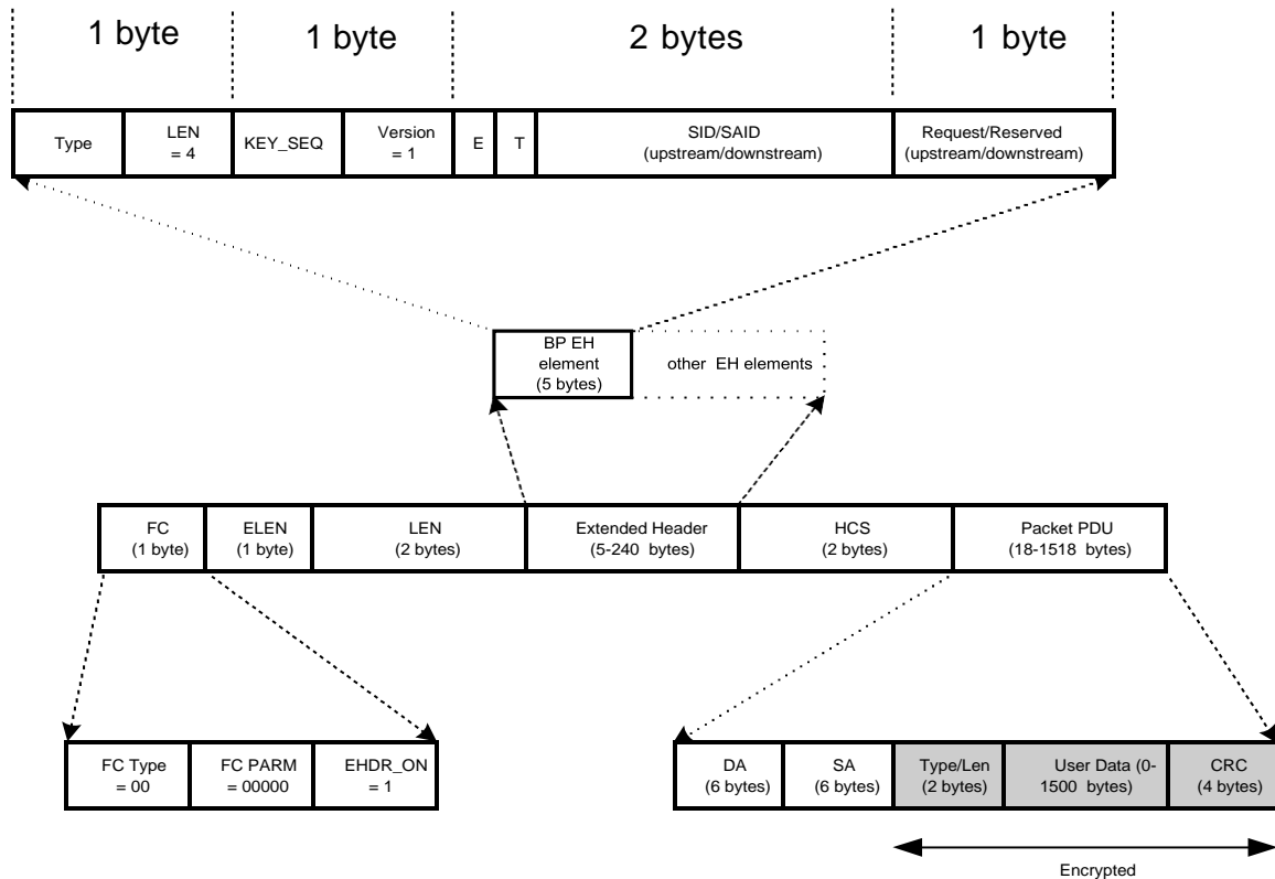
Figure 3-1. Format of DOCSIS Variable-length Packet Data PDU with Privacy EH Element
