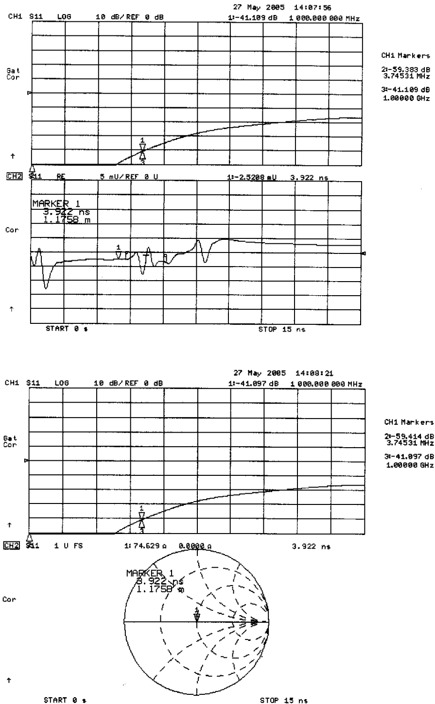
Figure 9 - Cable Impedance (Plots are for reference only. Displayed frequency settings may vary based on user test set up and requirements.)
