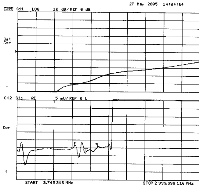
Figure 5 - Open End of Airline Adapter (Plots are for reference only. Displayed frequency range settings may vary based on user test set up and requirements.)
