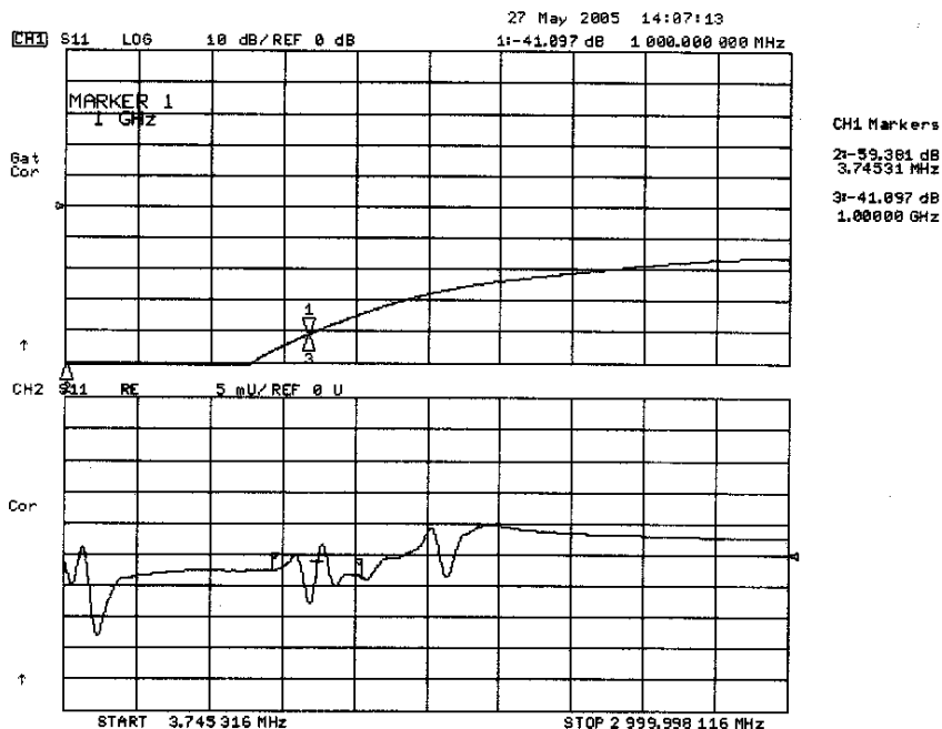
Figure 8 - Worst Case Return Loss (Plots are for reference only. Displayed frequency range settings may vary based on user test set up and requirements.)
