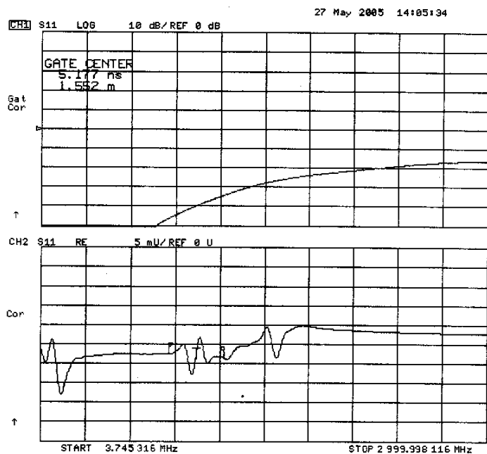
Figure 7 - Adjust Gate to Center DUT (Plots are for reference only. Displayed frequency range settings may vary based on user test set up and requirements.)
