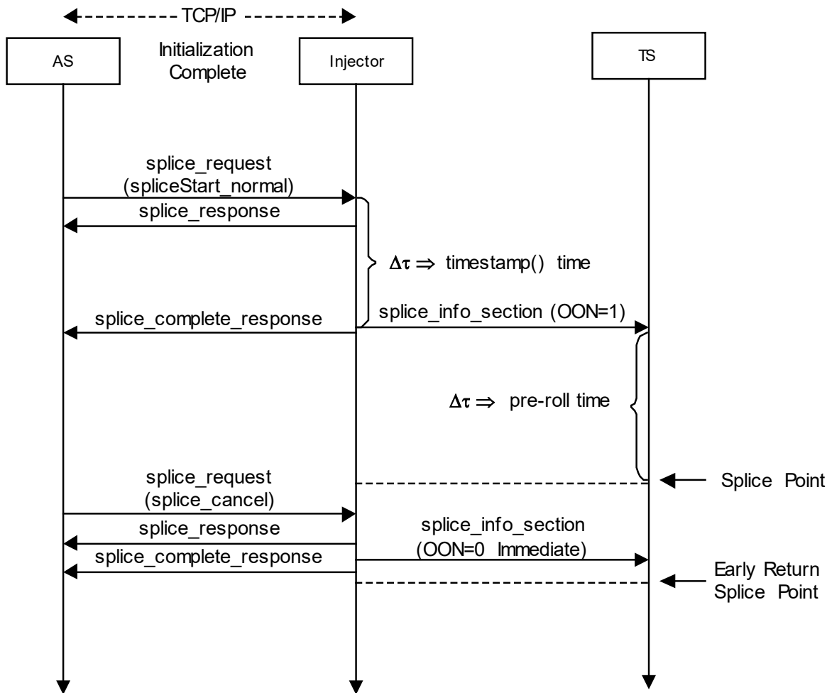
Figure 13-13: Two-way Flow Diagram Cancel after Splice Point
