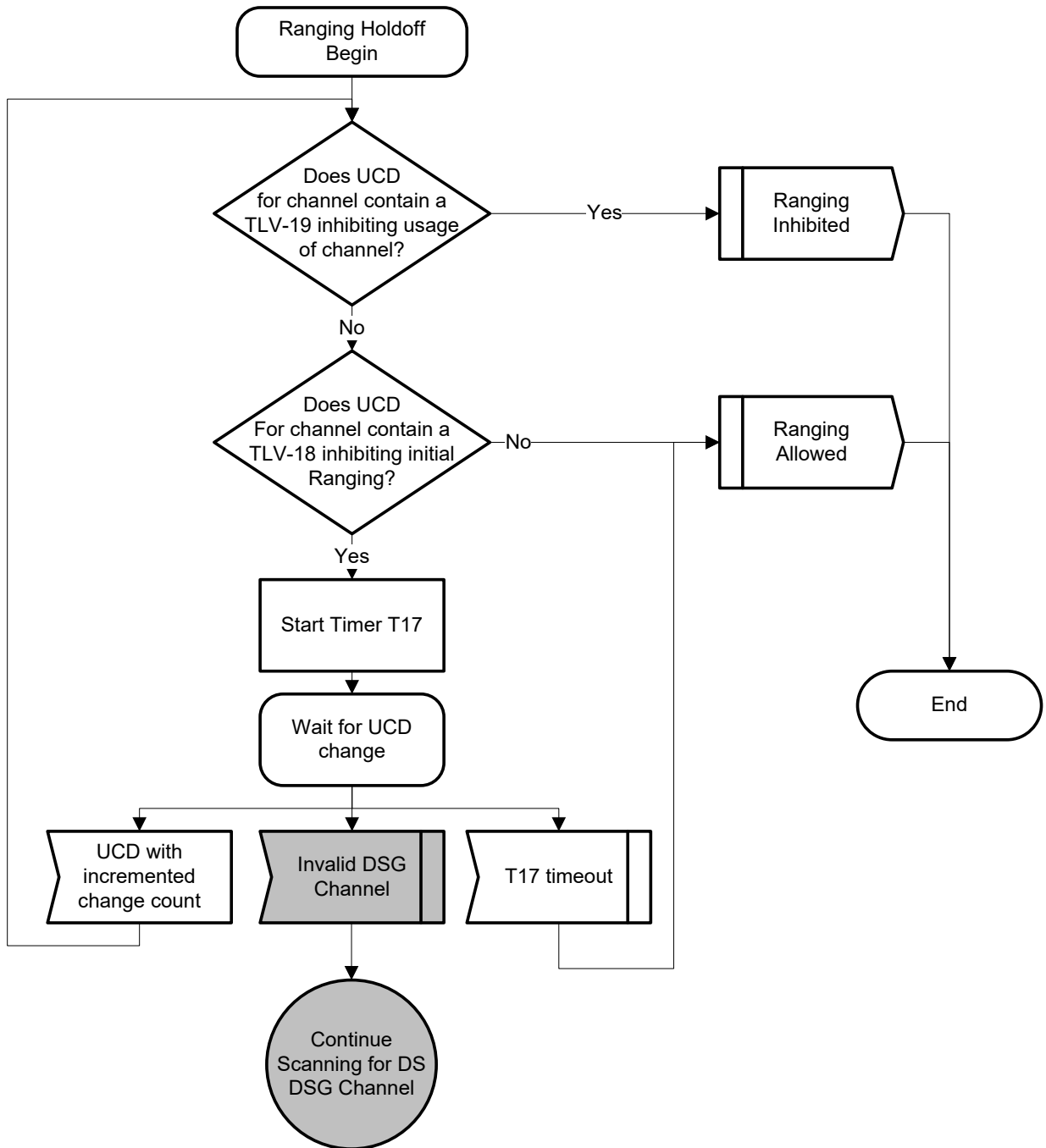
Figure 5-20 - Determine Ranging Hold-Off
