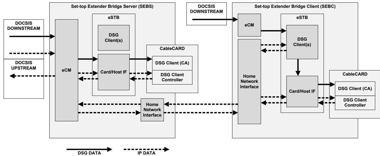
Figure F-1 - Block diagram of DSG SEB Solution
