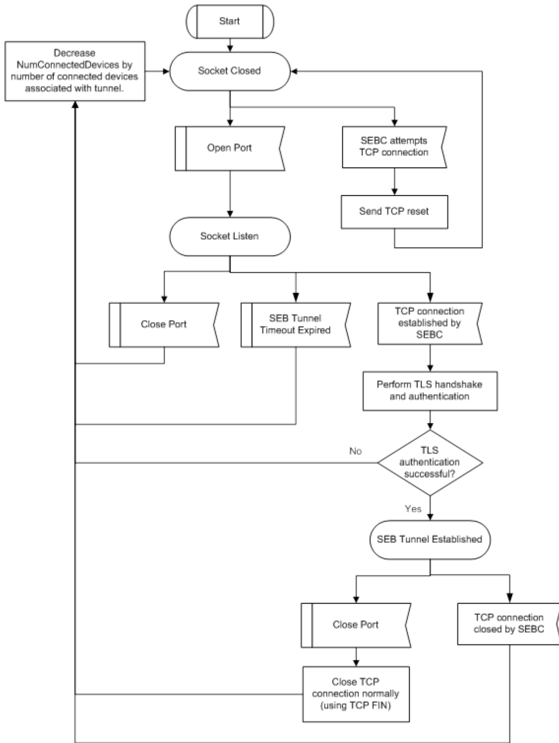
Figure F-9 - SEB Tunnel TCP Socket Handling
