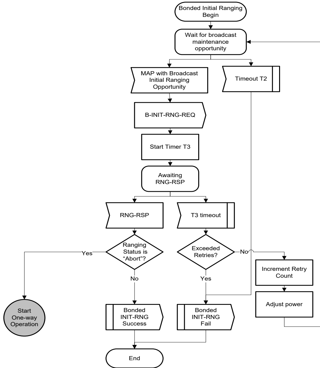
Figure 5-21 - Determine MD-US-SG
