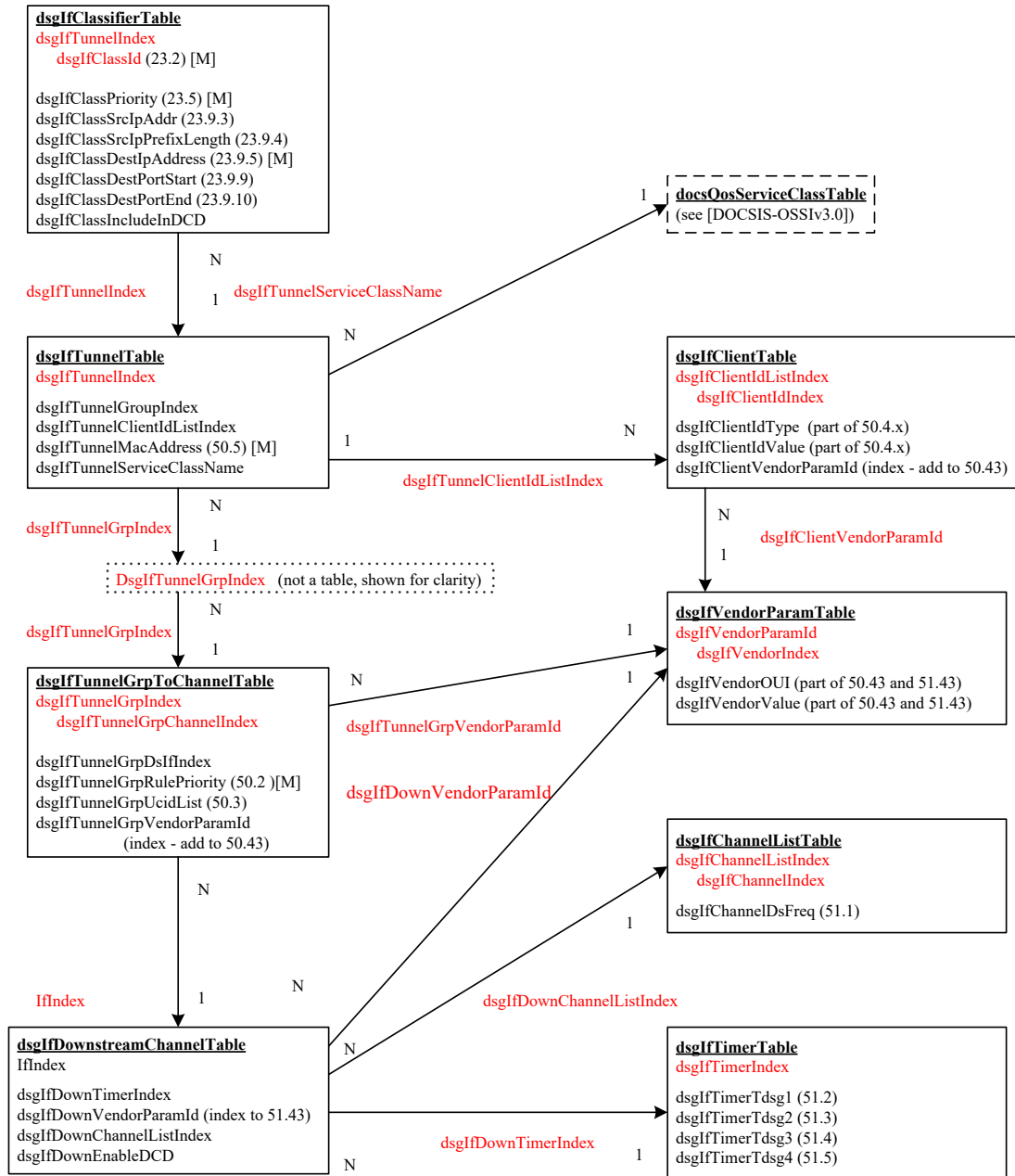
Figure I-1 - MIB Structure
