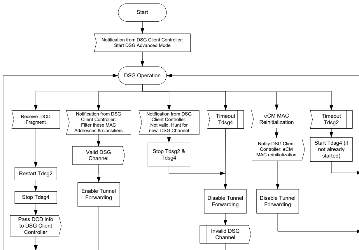
Figure 5–11 - DSG Operation
