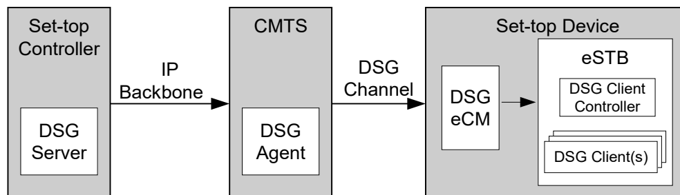
Figure 3-1 - DSG Terminology
