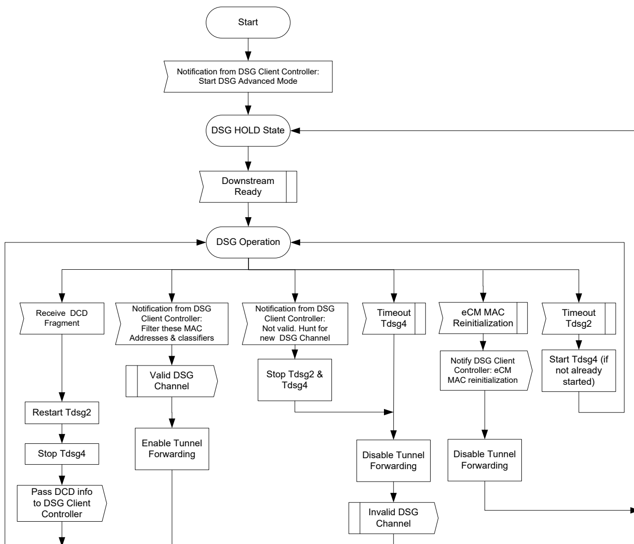
Figure 5–30 - DOCSIS 3.0 DSG Operation
