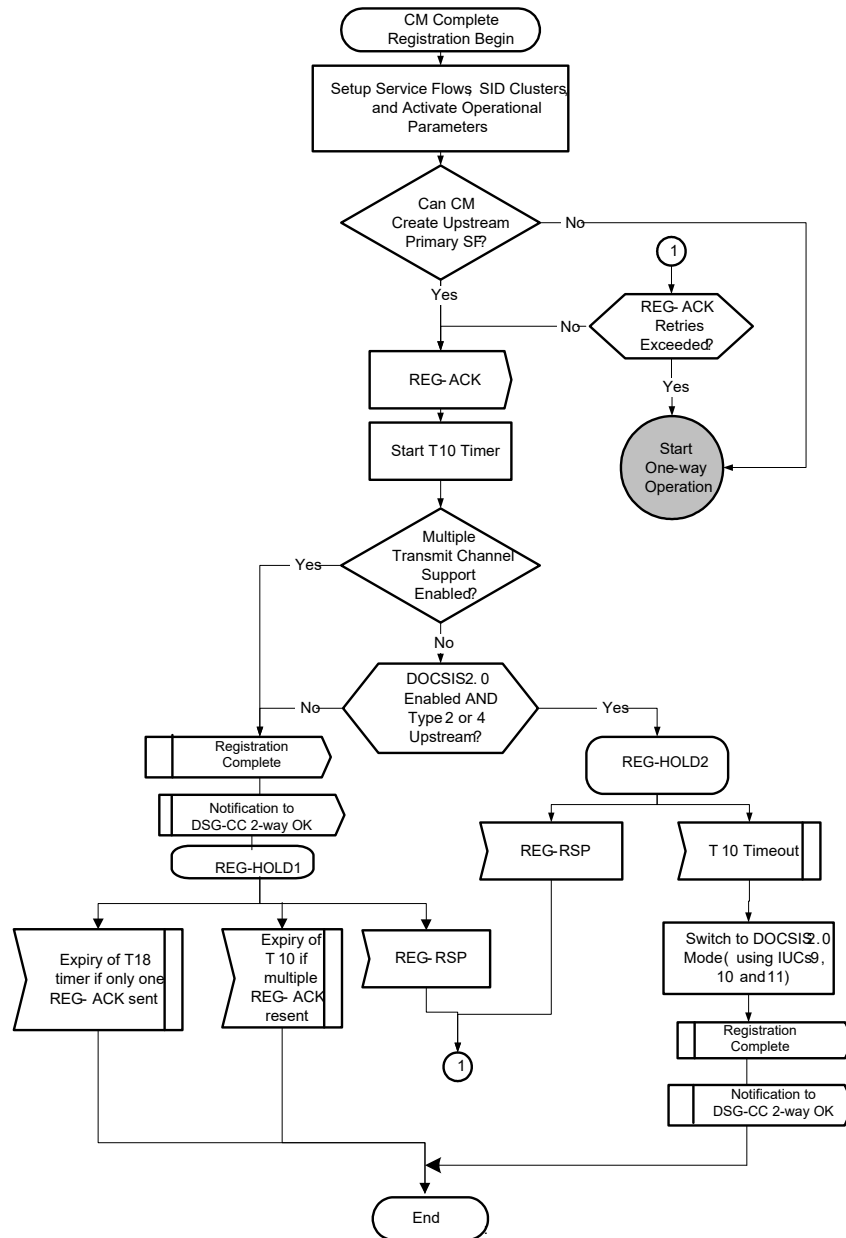
Figure 5-27 - CM Completes Registration
