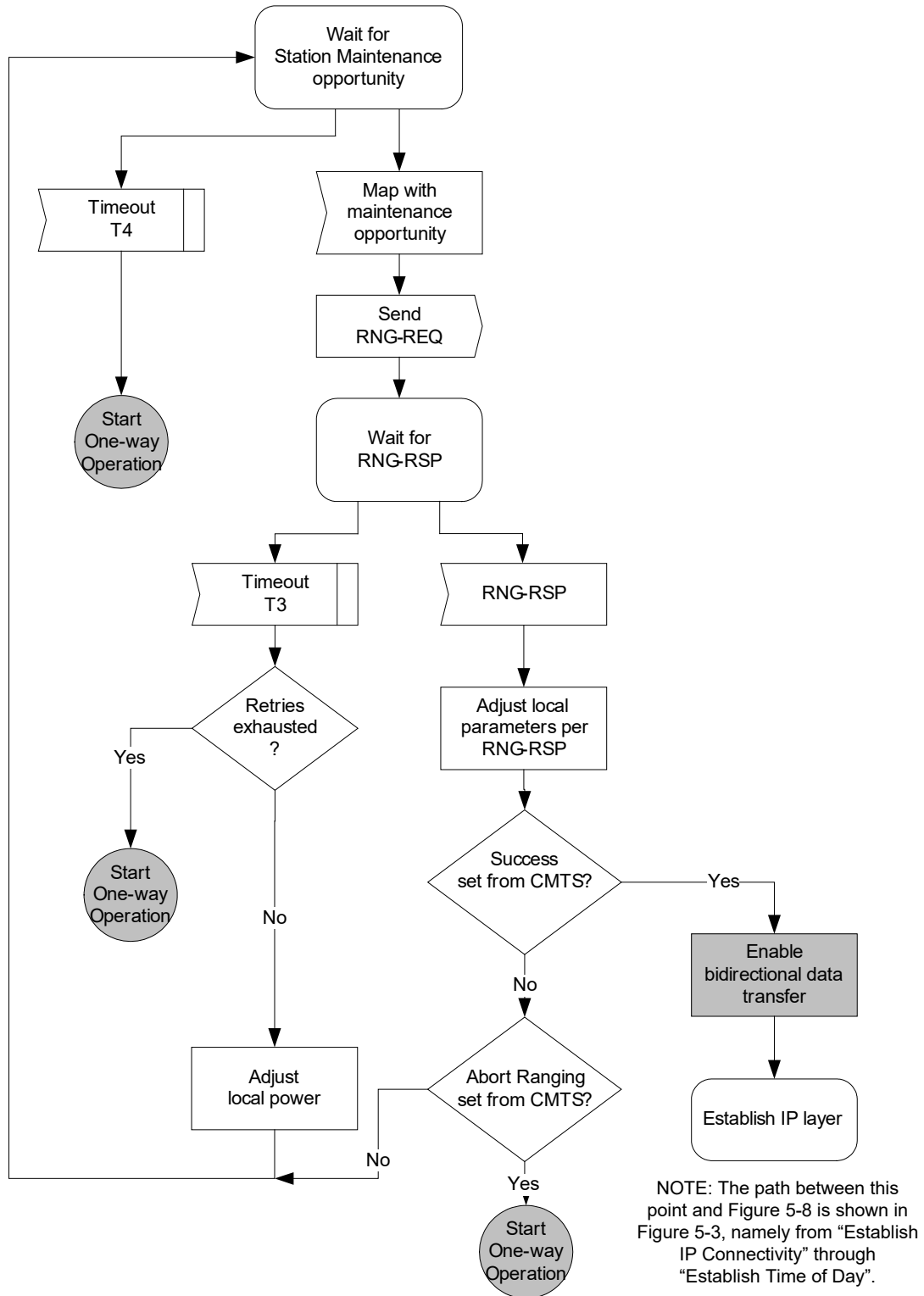
Figure 5-7 - DSG eCM Unicast Station Maintenance Ranging
