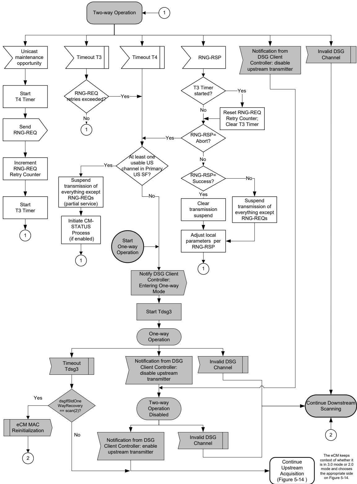
Figure 5-28 - eCM Operation
