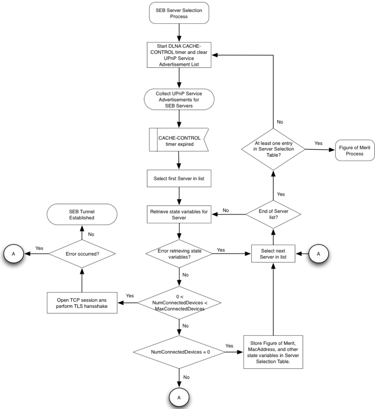
Figure F-5 - SEB Server Selection Process
