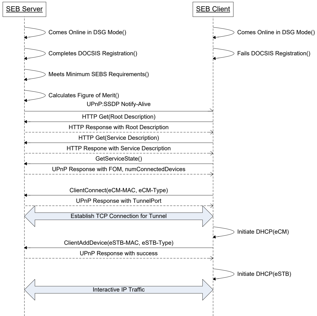
Figure F-3 - Basic SEBS and SEBC configuration
