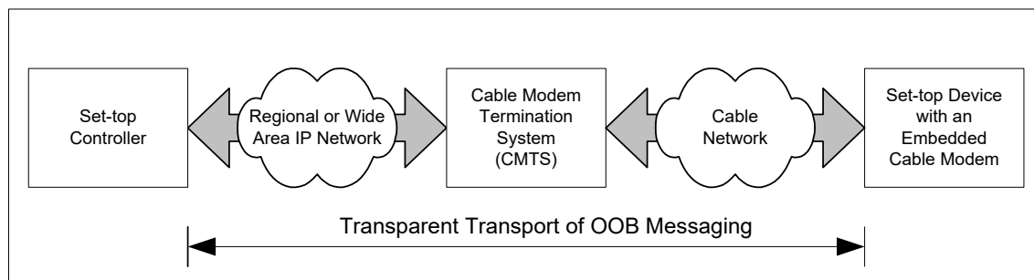
Figure 1-1 - Transparent Out-Of-Band Messaging Via DOCSIS
