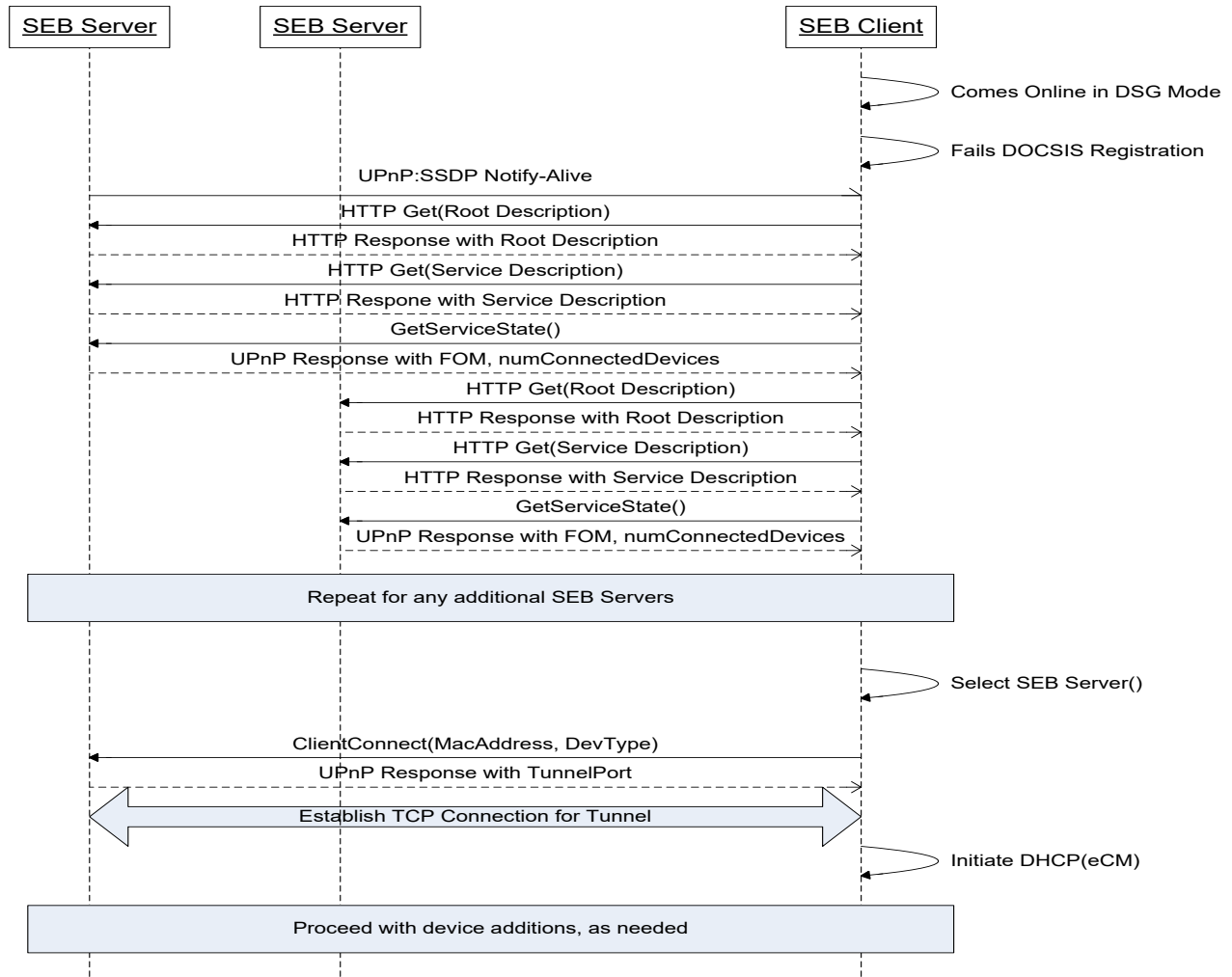
Figure F-4 - SEBS and SEBC configuration with Multiple SEBS Candidates
