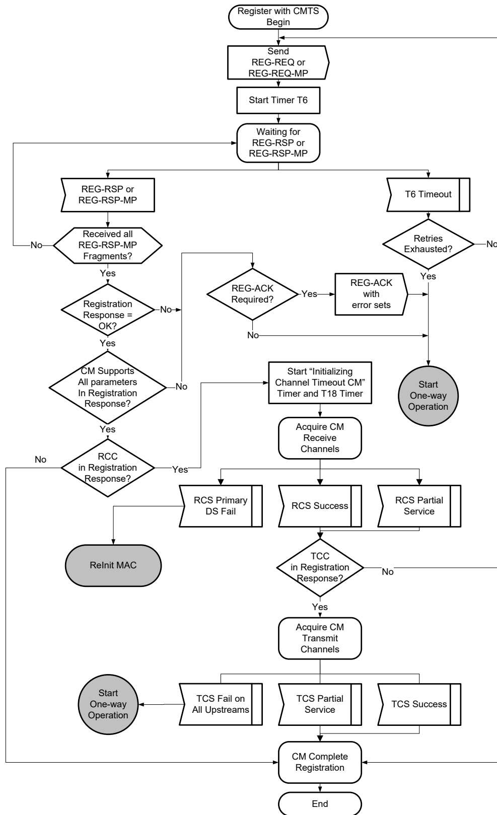
Figure 5-26 - CM Registration with CMTS
