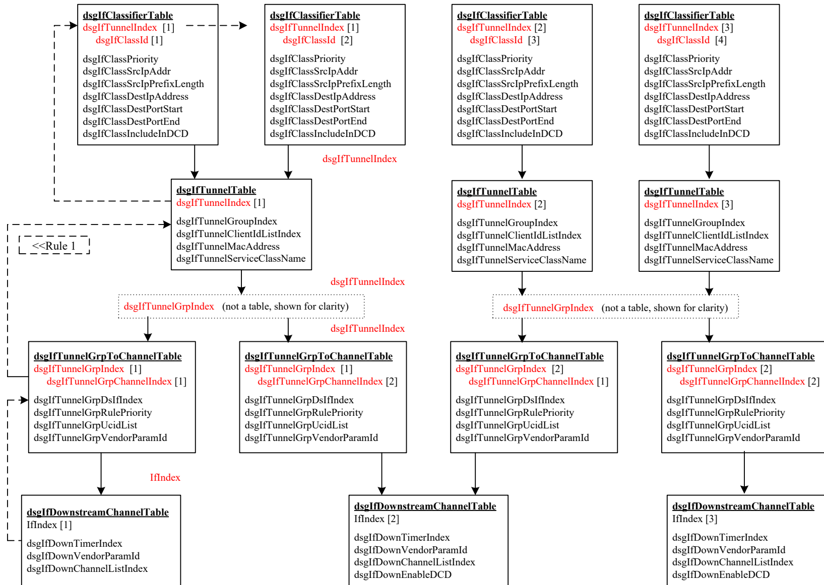
Figure I-3 - DS 1, Rule 1
