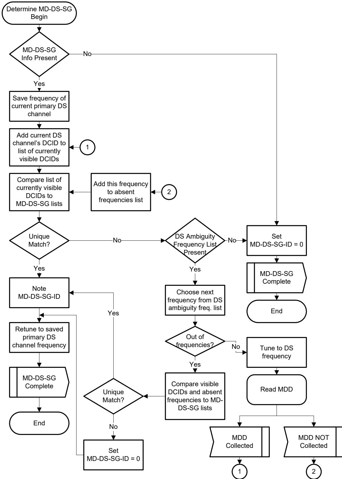
Figure 5-17 - Determine MD-DS-SG
