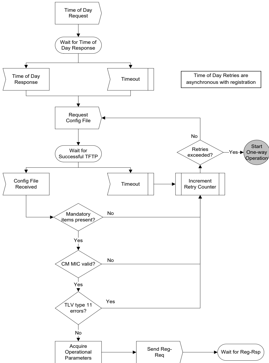
Figure 5-8 - DSG eCM Registration
