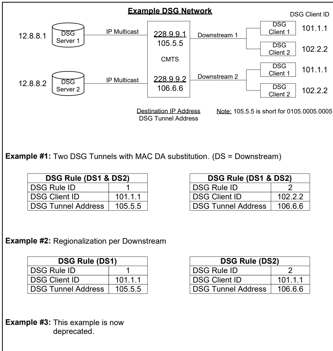
Figure 5-31 - Example DSG Configurations
