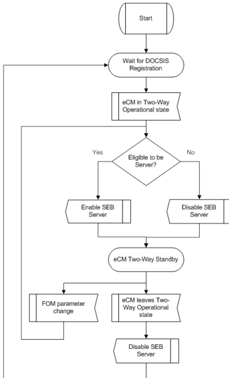
Figure F-7 - SEB Server Enable/Disable State
