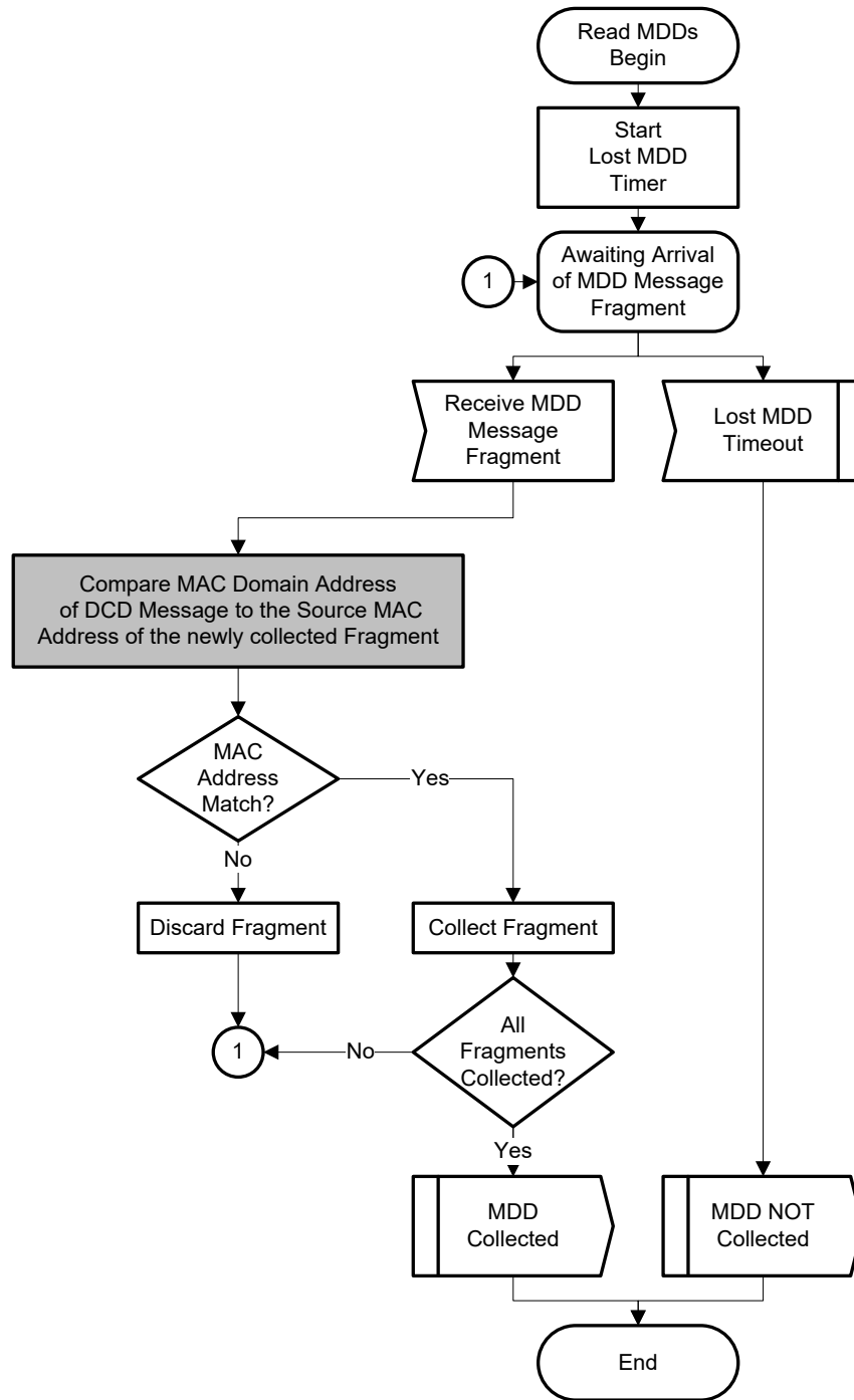
Figure 5-16 - Read MDD
